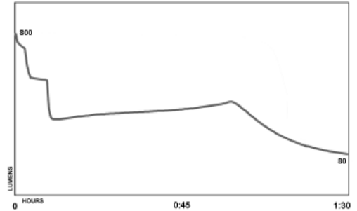
TAC-540XL PERFORMANCE CURVE
